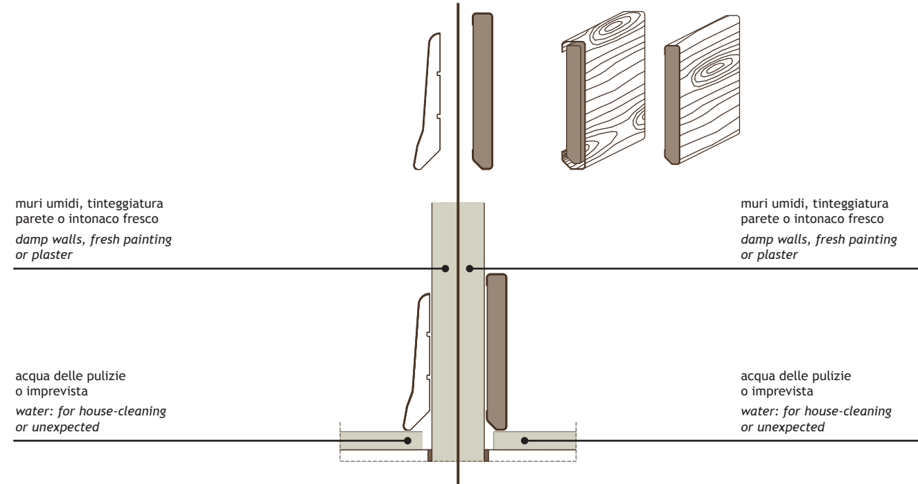
BATTISCOPA STANDARD STANDARD BASEBOARD
