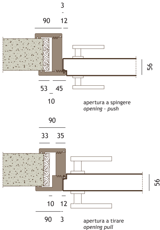
incastro coprifilo/ stipite a pettine brevetto Pivato finger-joint snap-fitting between casing and jamb, Pivato patented
